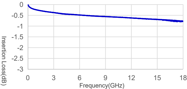
A81-NMNWM-1m Insertion Loss
