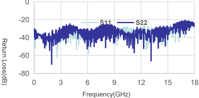
A81-NMNWM-1m Return Loss
